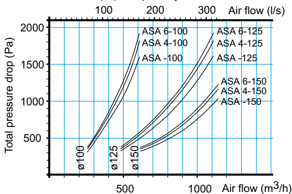
Pressure drop (completely extended hose, 5 m)
