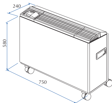
INDOOR UNIT
