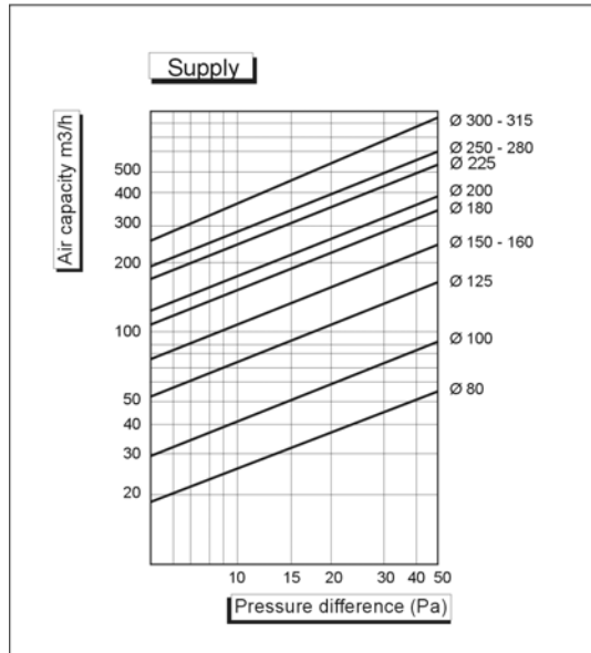
PRESSURE LOSS DIAGRAM
